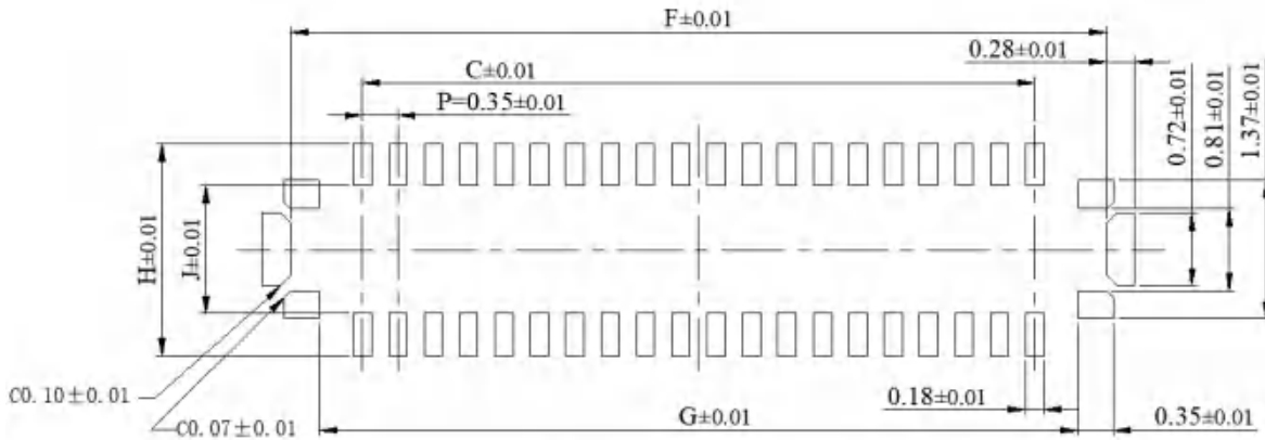
RECOMMENDED METAL DIMENSIONS (THICKNESS: 0.08 mm)
